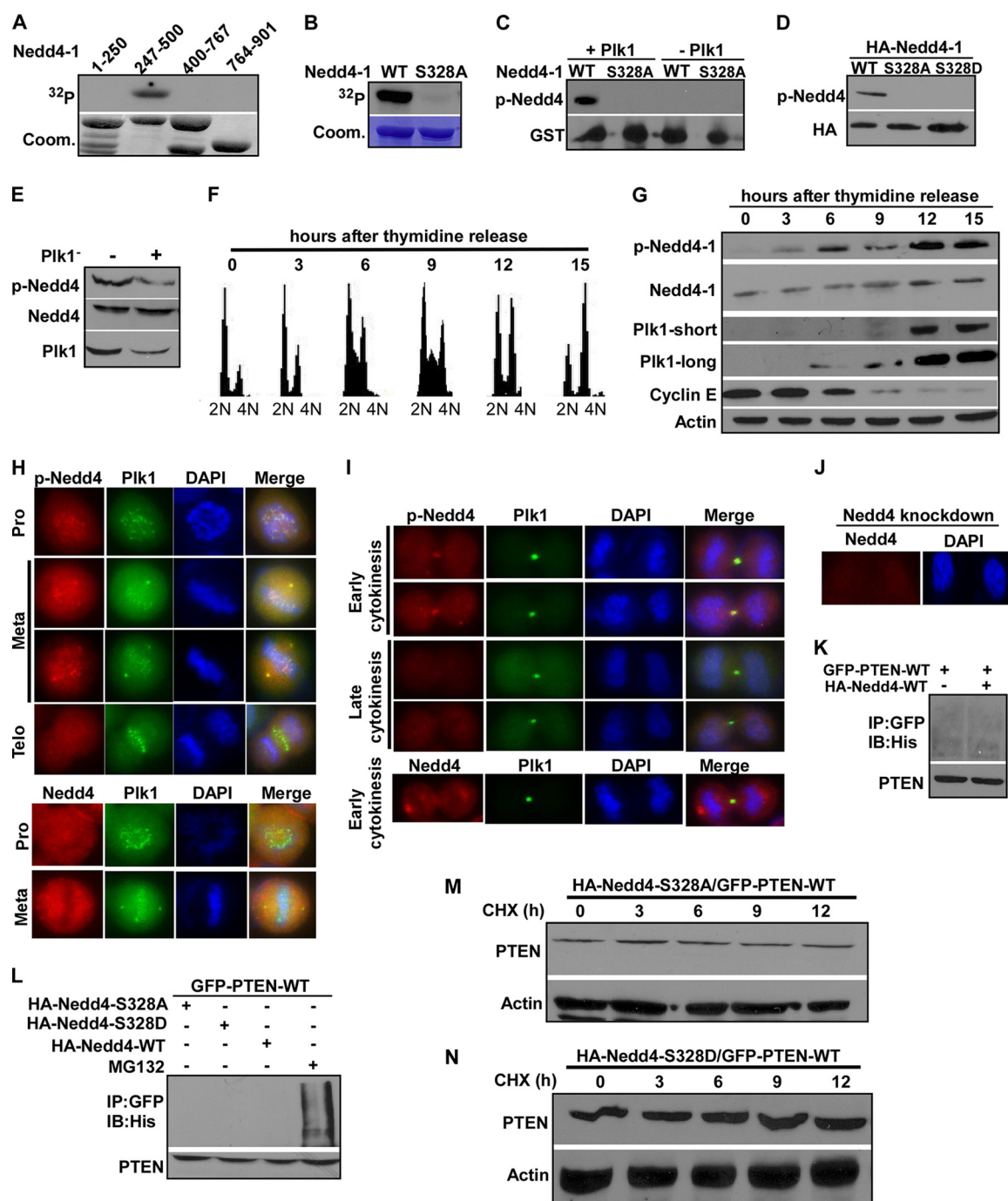
FIG 10 Plk1 targets Nedd4-1 at S328. (A and B) Plk1 phosphorylates Nedd4-1-S328. Plk1 was incubated with GST-Nedd4-1 regions (A) or different mutants (B) as for Fig. 3B. (C) The pS328-Nedd4-1 antibody is specific. Plk1 was incubated with GST-Nedd4-1 in the presence of unlabeled ATP. (D) Nedd4-1-S328 is phosphorylated in vivo . 293T cells were transfected with Nedd4-1 constructs for 48 h. (E) Endogenous Plk1 phosphorylates endogenous Nedd4-1 at S328. 293T cells were depleted of Plk1 by RNAi for 48 h. (F and G) Phosphorylation of Nedd4-1-S328 is cell cycle regulated. HeLa cells were subjected to a double thymidine block (16 h of thymidine treatment, 8 h of release, and a second thymidine block for 16 h), released for different times, and harvested for FACS analysis (F) or IB (G). (H to J) Colocalization of pNedd4-1 and Plk1 at mitotic structures. HeLa cells were subjected to IF staining with the indicated antibodies. Pro, prophase; Meta, metaphase; Telo, telophase. (K to N) Phosphorylation of Nedd4-1-S328 does not affect its E3 ubiquitin ligase activity toward WT-PTEN. (K) 293T cells were cotransfected with GFP-PTEN, HA-Nedd4-1, and His-ubiquitin and harvested for anti-GFP IP, followed by anti-His IB. (L) 293T cells were cotransfected with the indicated plasmids, treated with MG132 or left untreated, and harvested for anti-GFP IP, followed by anti-His IB. (M and N) 293T cells were cotransfected with the indicated plasmids, treated with cycloheximide for different times, and harvested for IB.
